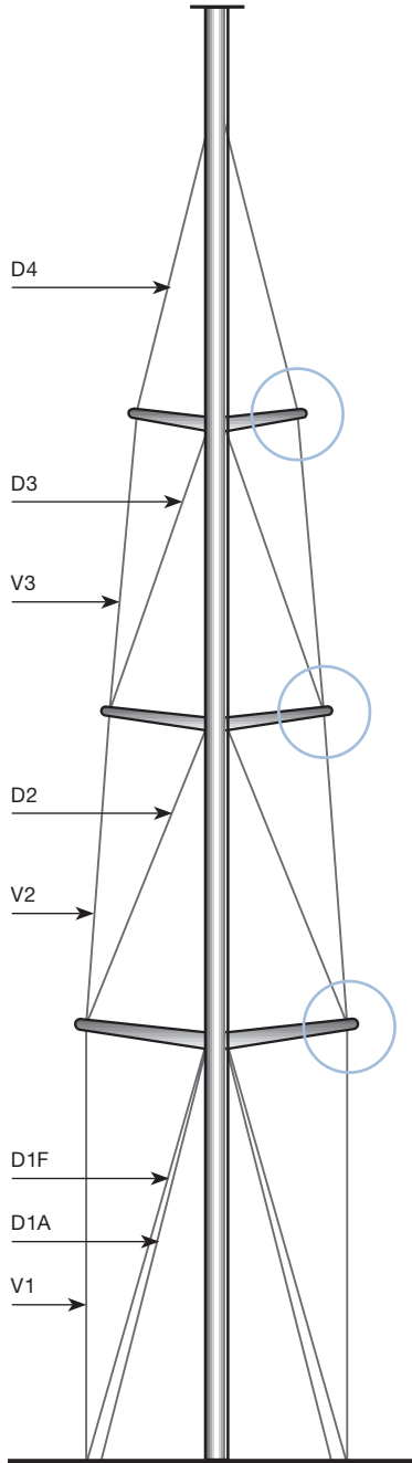
Linked rigging.
