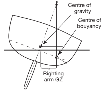
Righting moment = GZ x displacement.
