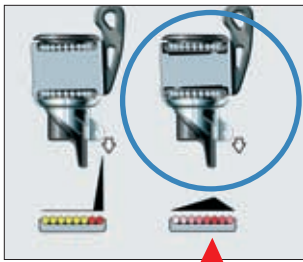
Seldén patented load distributor.
